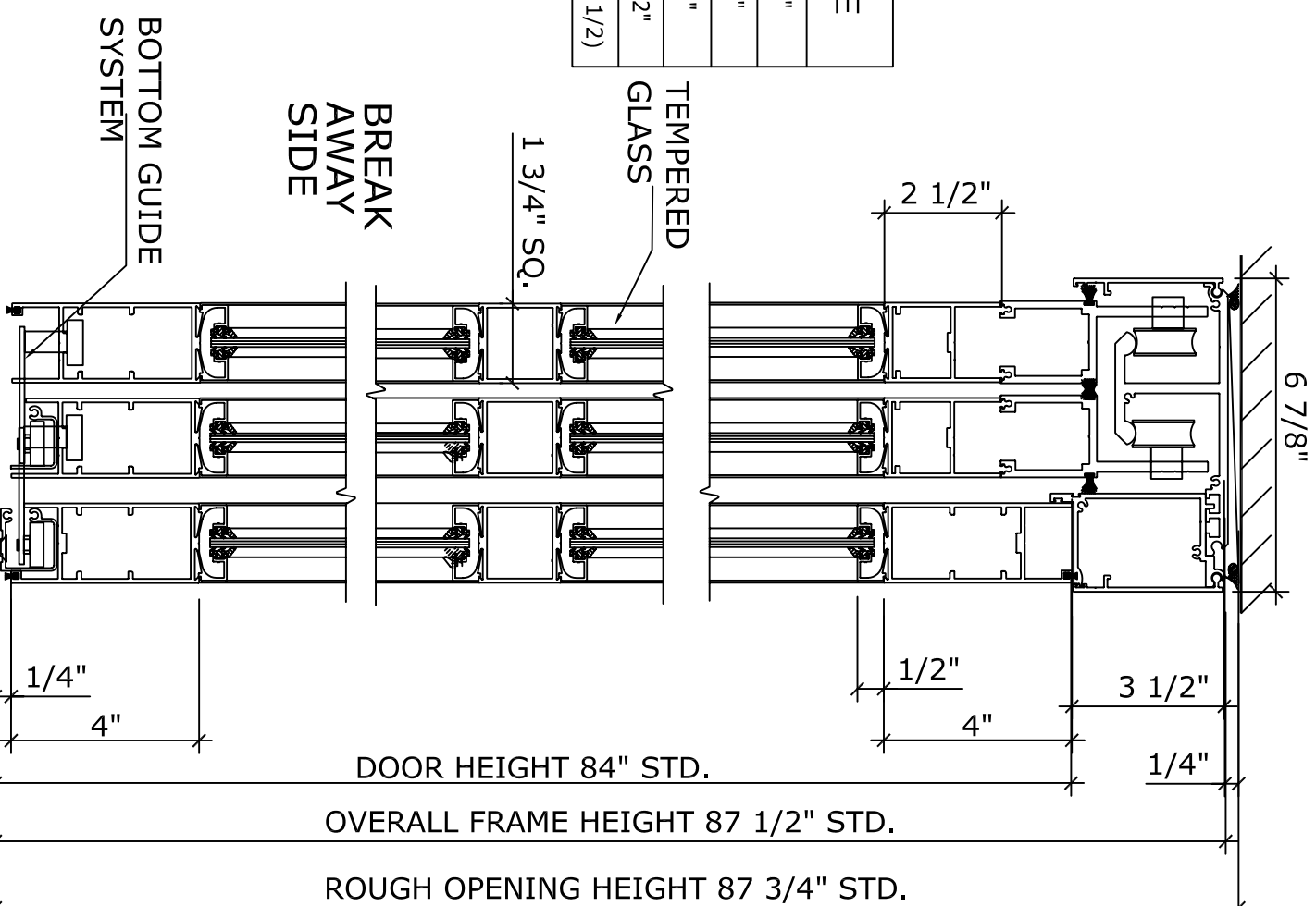
2 VERTICAL SECTION
